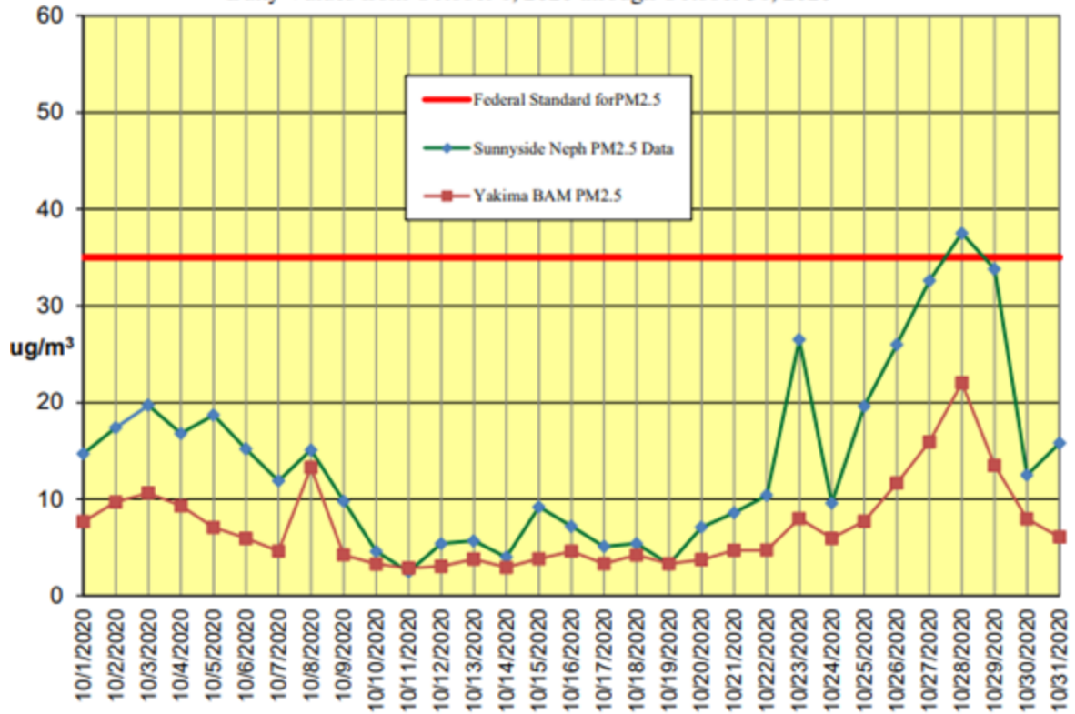
Monthly PM 2.5 Data for Yakima & Sunnyside Daily Values from October 1, 2020 through October 31, 2020
